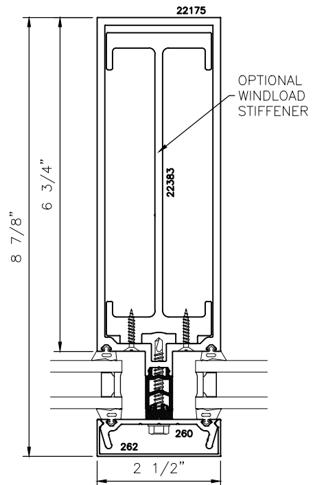
OPT. 5.4
