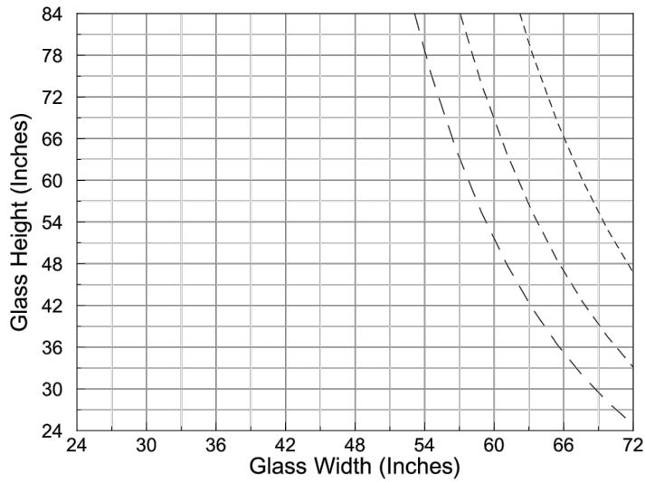
Deadload chart for #452
