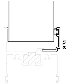
SILL
