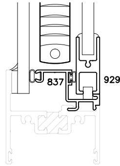
SILL
