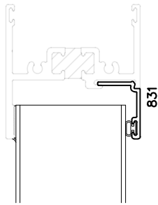
HEAD
